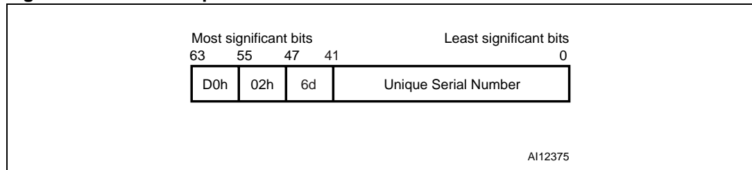
Figure 50. 64-bit Unique Identifier of the SRI512
