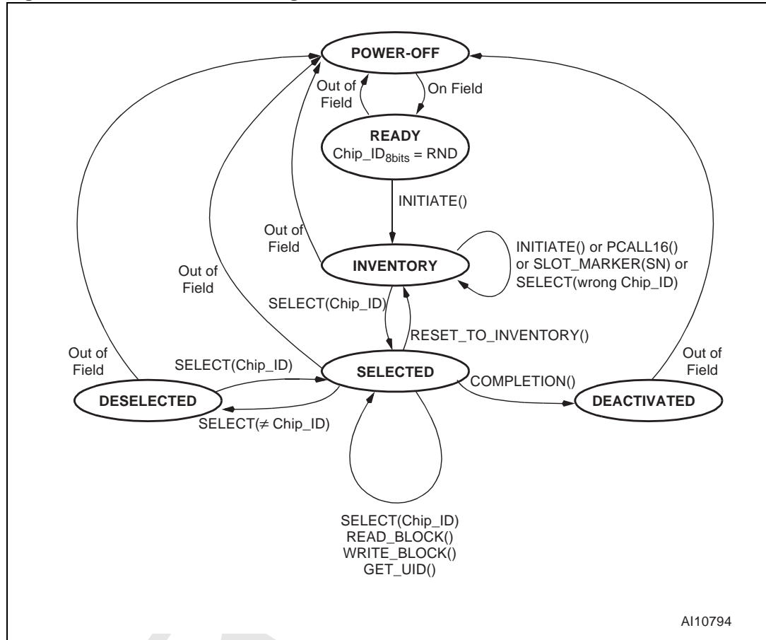
Figure 20. State Transition Diagram
