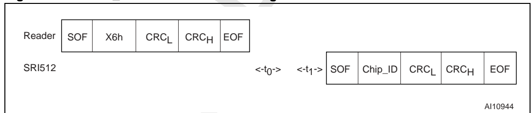
Figure 58. SLOT_MARKER Frame Exchange Between Reader and SRI512
