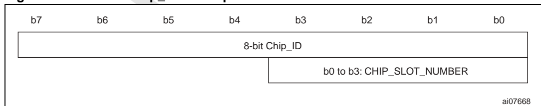
Figure 21. SRI512 Chip_ID Description
