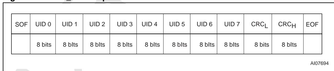
Figure 49. GET_UID Response Format
