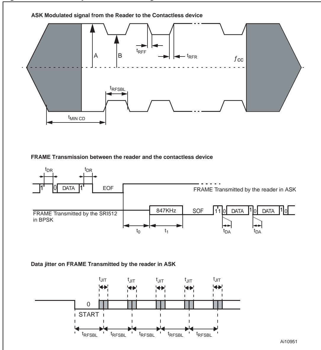
Figure 52. SRI512 Synchronous Timing, Transmit and Receive
