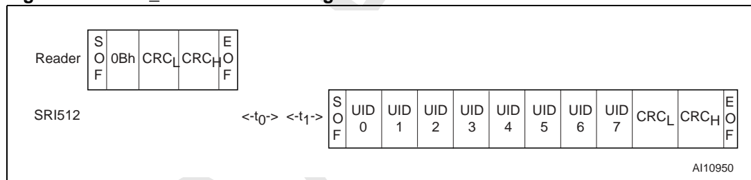
Figure 51. GET_UID Frame Exchange Between Reader and SRI512
