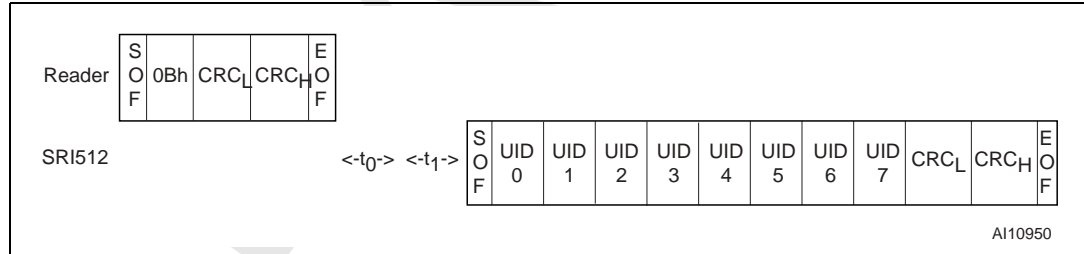
Figure 64. GET_UID Frame Exchange Between Reader and SRI512
