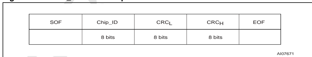
Figure 31. SLOT_MARKER Response Format
