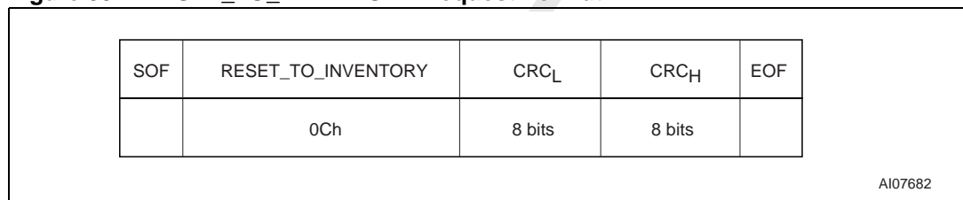
Figure 39. RESET_TO_INVENTORY Request Format
