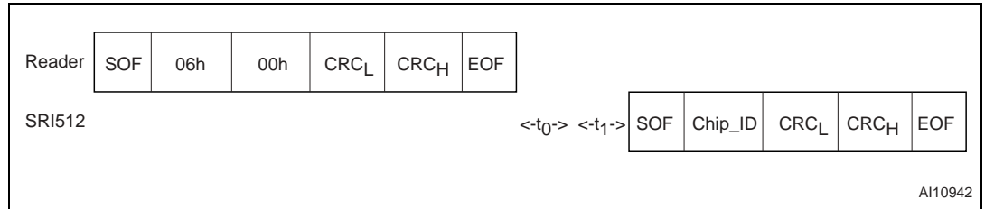
Figure 56. INITIATE Frame Exchange Between Reader and SRI512
