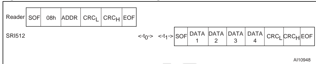
Figure 63. WRITE_BLOCK Frame Exchange Between Reader and SRI512
