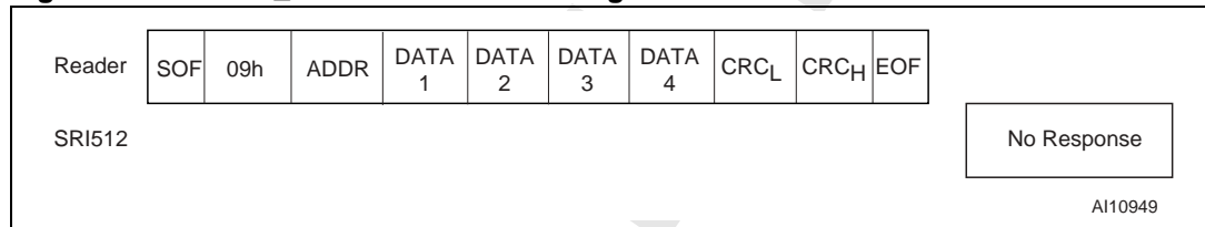
Figure 64. GET_UID Frame Exchange Between Reader and SRI512
