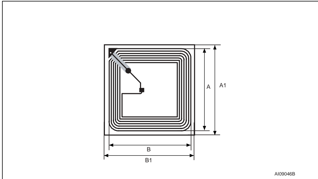
Figure 53. A3 Antenna Specification
