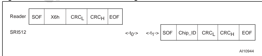
Figure 32. SLOT_MARKER Frame Exchange Between Reader and SRI512
