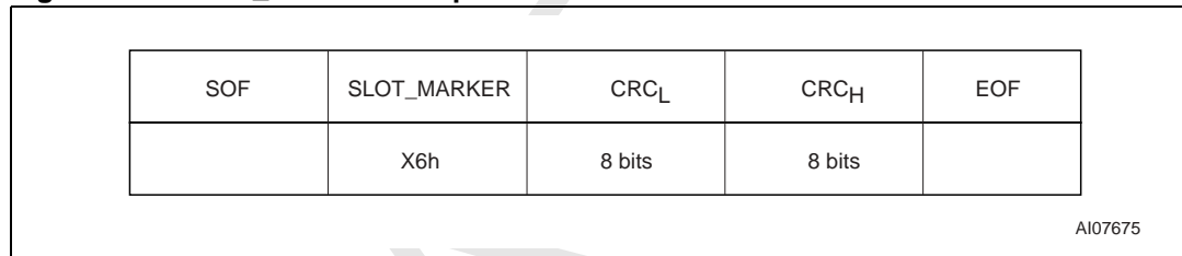
Figure 30. SLOT_MARKER Request Format
