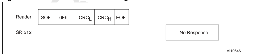
Figure 38. COMPLETION Frame Exchange Between Reader and SRI512
