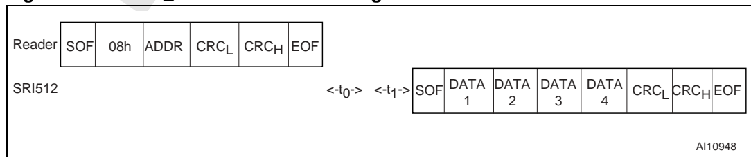
Figure 44. READ_BLOCK Frame Exchange Between Reader and SRI512
