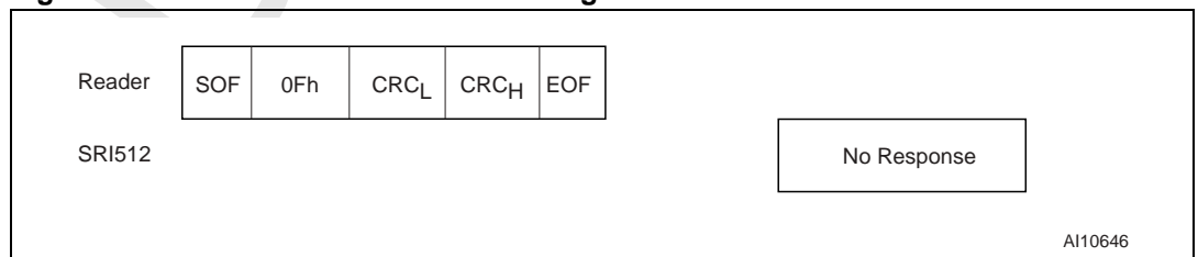
Figure 60. COMPLETION Frame Exchange Between Reader and SRI512
