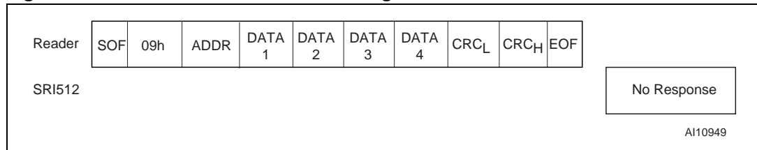
Figure 47. WRITE_BLOCK Frame Exchange Between Reader and SRI512
