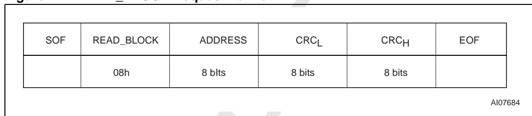
Figure 42. READ_BLOCK Request Format
